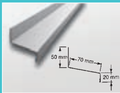
Droppbleck
